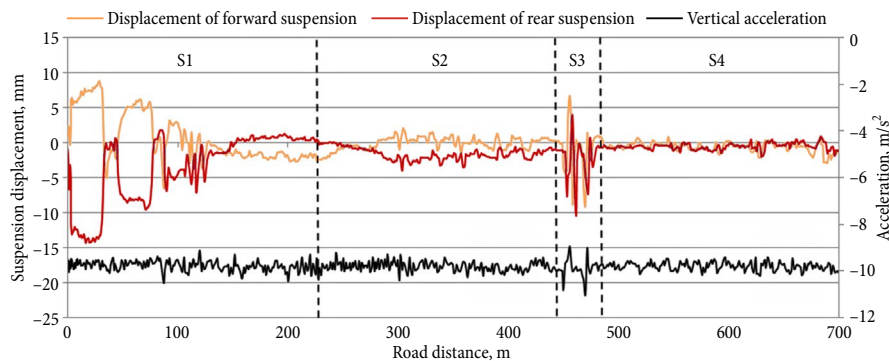
Fig. 5. Vehicle motions in vertical axis, v = 50 km/h
